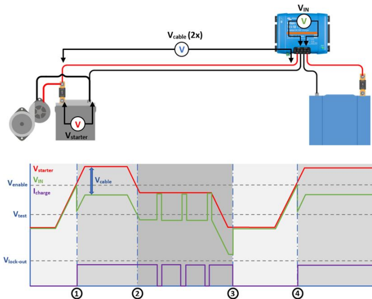
Figure 7: Engine on detection sequence
