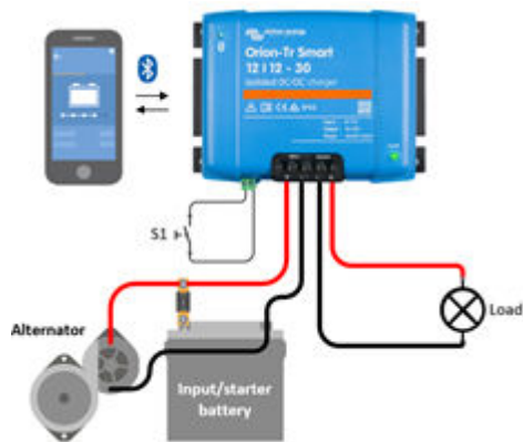
Figure 1: Typical connection setup as DC-DC converter
