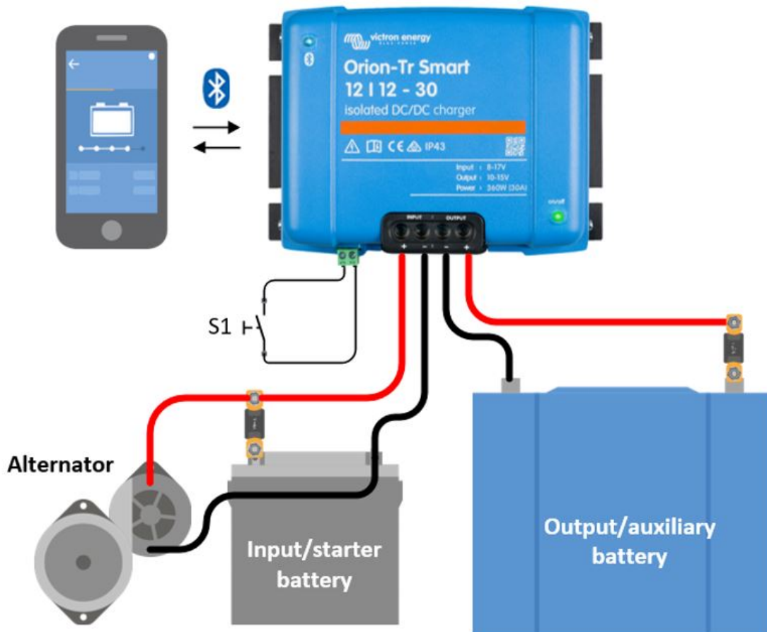
Figure 2: Typical connection setup as charger
