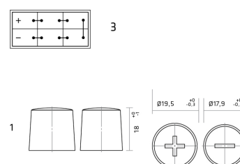
Layout
