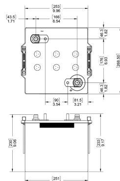
ODS-AGM6M DUAL TERMINALS (AUTOMOTIVE DIN TAPER POST AND MARINE STUDS)
