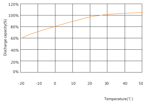
Discharge capacity vs. temperature
